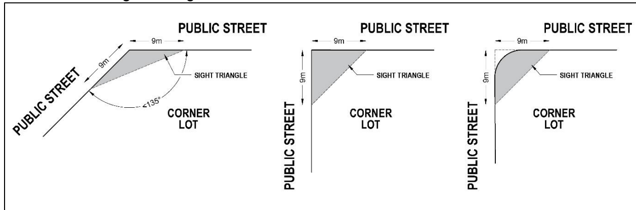
Illustration 9 – Sight Triangles
