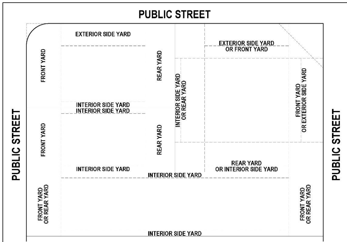
Illustration 4 - Yards
