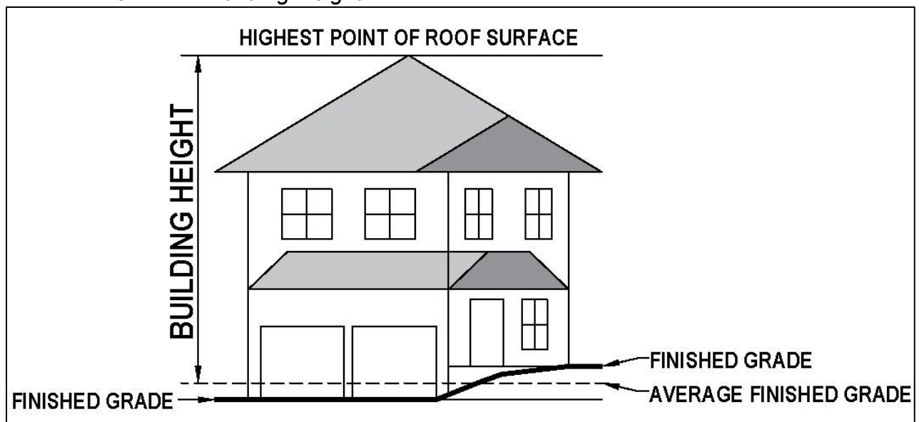
Illustration 6 – Main Building Height
